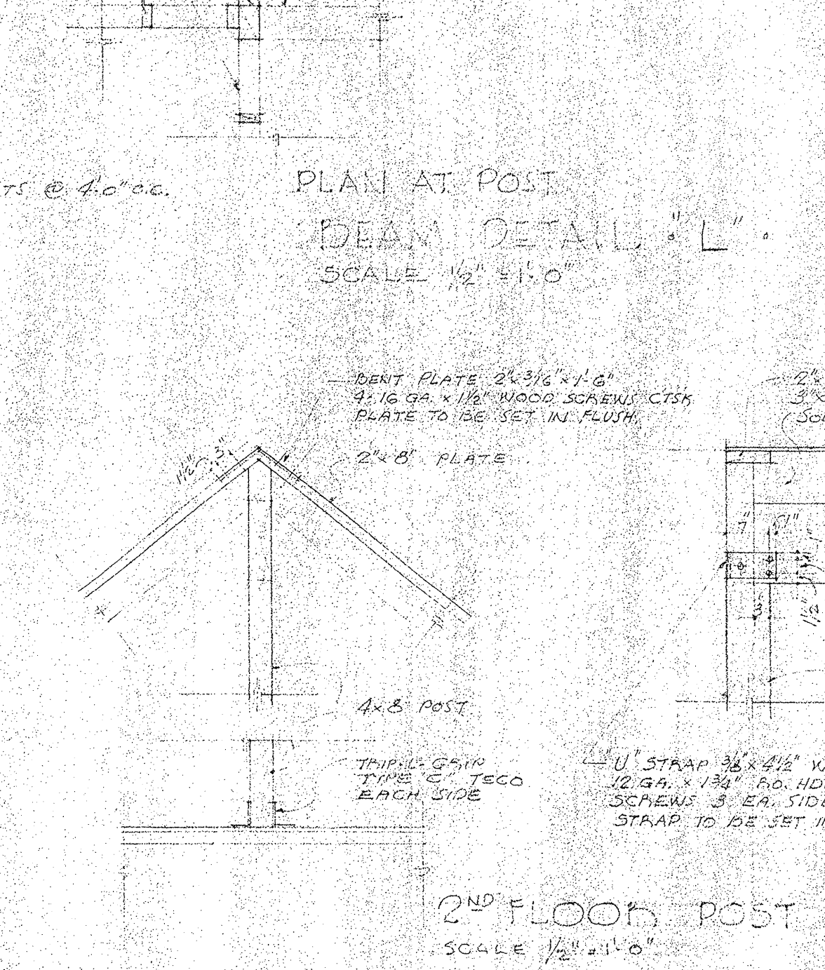
PLAN AT POST
