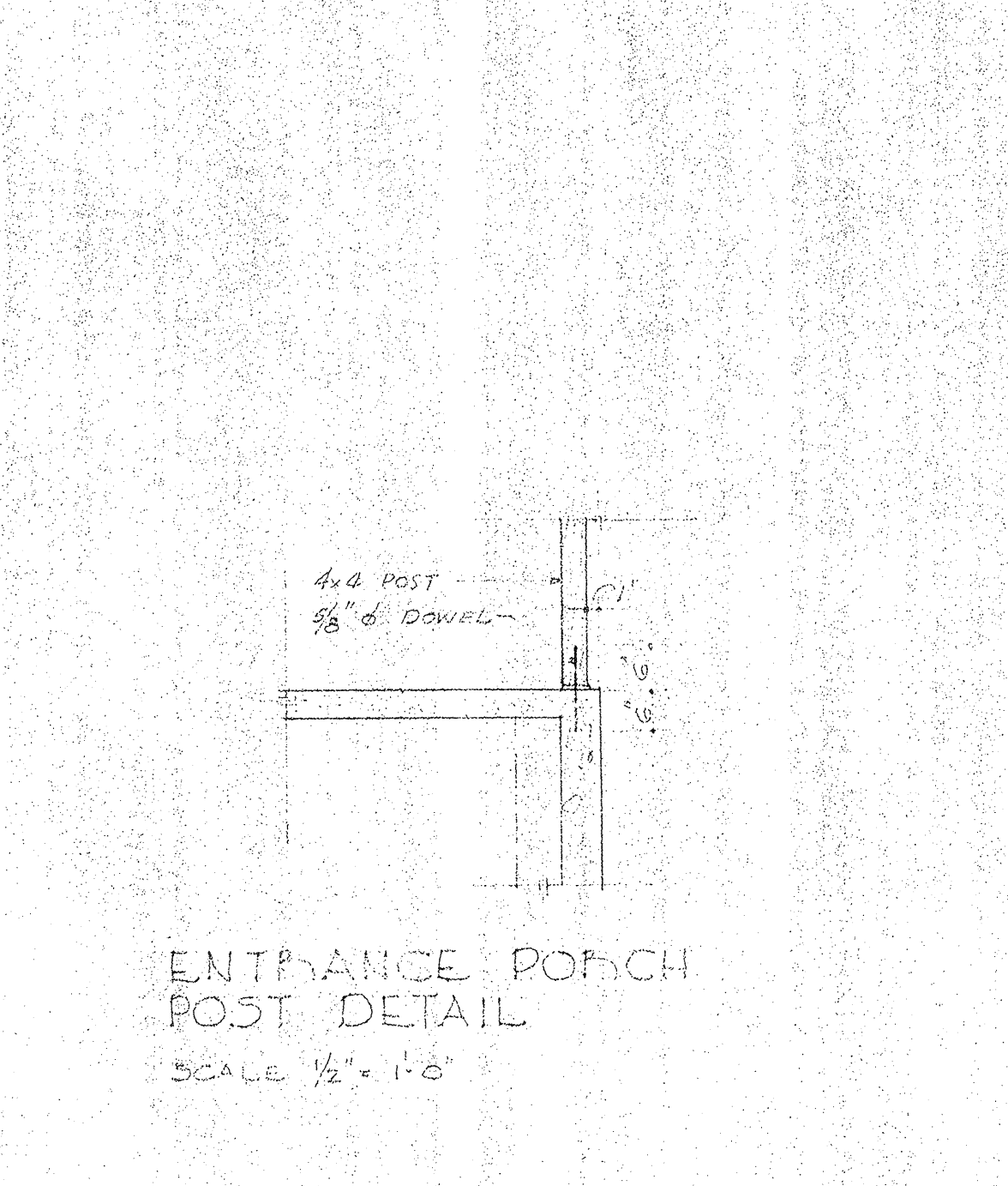
ENTRANCE PORCH POST DETAIL
